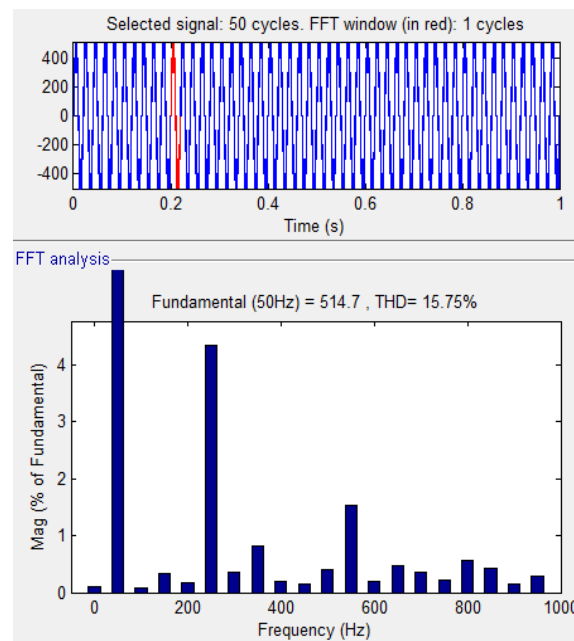
Fig.10. FFT Analysis of the harmonic spectrum for CO-PWM technique
