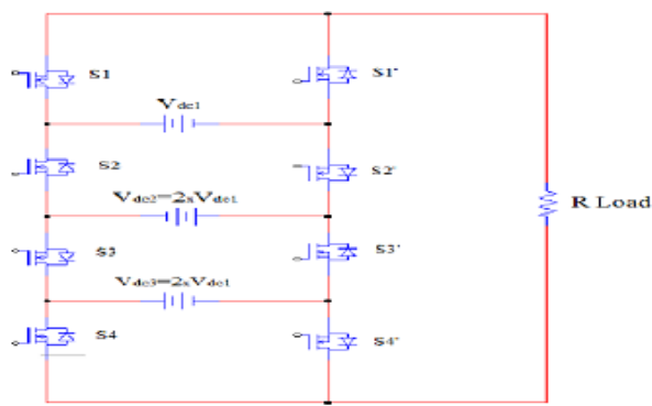
Fig.1 Proposed configuration for single phase inverter operation
