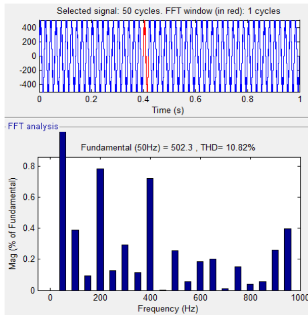
Fig.6. FFT Analysis of the harmonic spectrum for IPD-LSPWM technique
