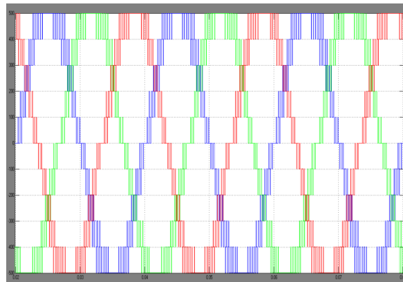
Fig.9. Output voltage waveform for three phase 11 level Inverter using CO-PWM technique
