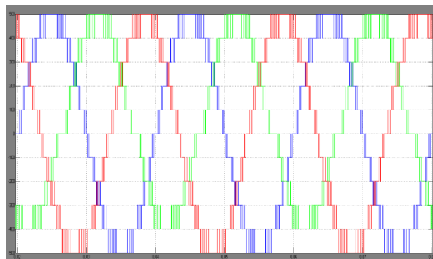
Fig.7. Output voltage waveform for three phase 11 level Inverter using APDLSPWM technique.
