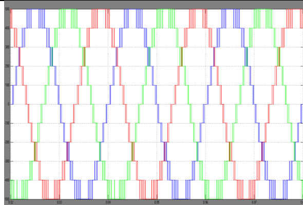
Fig.14. Output voltage waveform for three phase 11 level inverter using IPD-LSPWM technique with grid connected solar system
