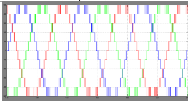
Fig.5. Output voltage waveform for three phase 11 level inverter using IPD-LSPWM technique
