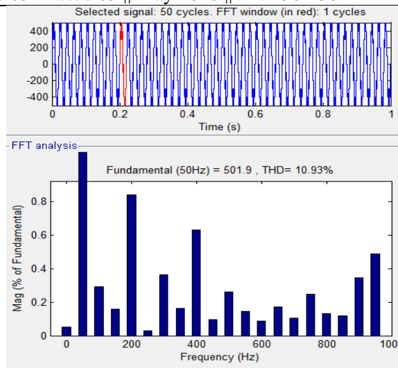
Fig.8. FFT Analysis of the harmonic spectrum for APD-LSPWM technique
