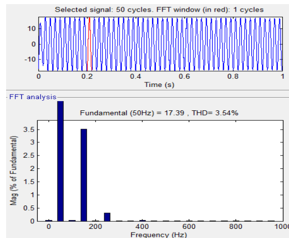
Fig.17. FFT Analysis of the harmonic spectrum for IPD-PWM technique with grid connected solar system.
