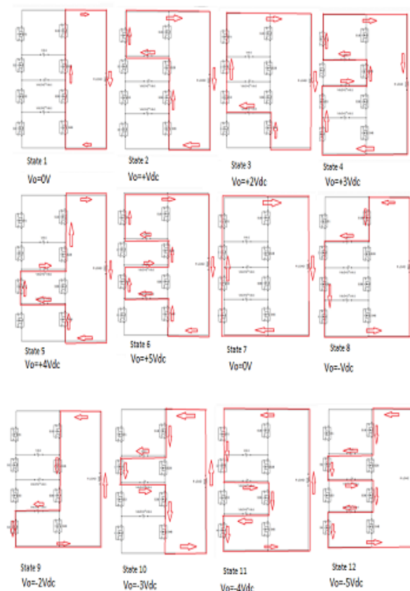
Fig.2. States corresponding to each Output voltage level
