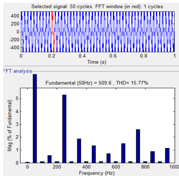
Fig.12. FFT Analysis of the harmonic spectrum for VF-PWM technique
