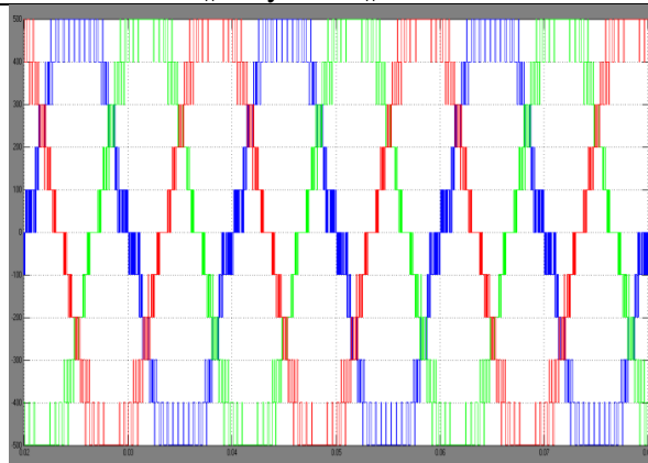
Fig.11. Output voltage waveform for three phase 11 level Inverter using VF PWM technique
