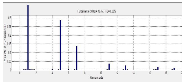
Fig 9. Harmonic analysis at 78 rad/sec for (i) No filter (ii) shunt active filter (iii) hybrid filter
