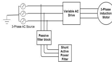
Fig. 2 Block diagram of hybrid filter
