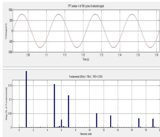
Fig. 12 Voltage waveform and THD with Hybrid filter at 78 rad/sec
