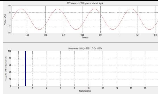
Fig. 11 Voltage waveform and THD with active filter at 78 rad/sec.
