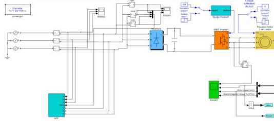
Fig.5 Simulation model with Shunt APF
