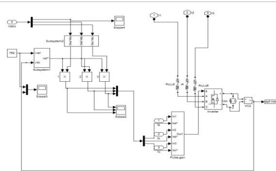
Fig.6 Shunt APF model with PI Controller
