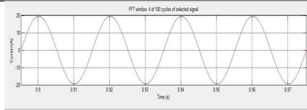
Fig. 8 Current waveform at 78 rad/sec for (i) no filter (ii) shunt active filter (iii) hybrid filter
