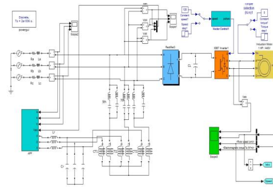
Fig. 7 Simulink model of Hybrid filter
