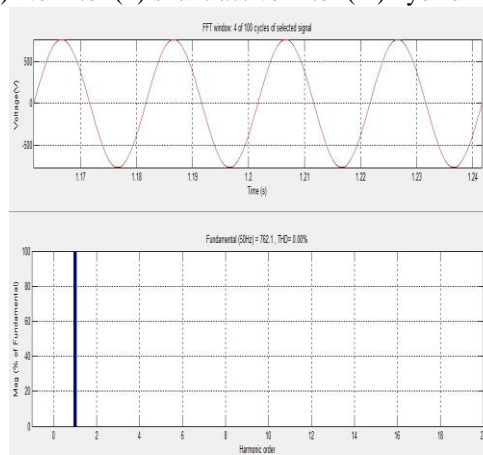
Fig. 10 Voltage waveform and THD with no filter at 78 rad/sec
